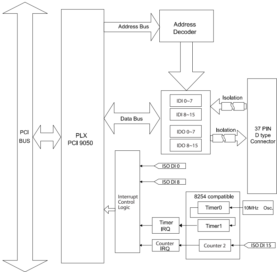
Figure 2.2 Block Diagram
