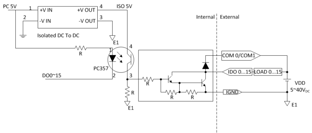
Figure 3.2 Connecting an external output load
